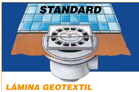
VÁLVULA PLATO DE DUCHA OBRA STANDARD GEOTEXTIL "GEO-TEXTILE" VALVE FOR BUILDING SHOWER BASE
